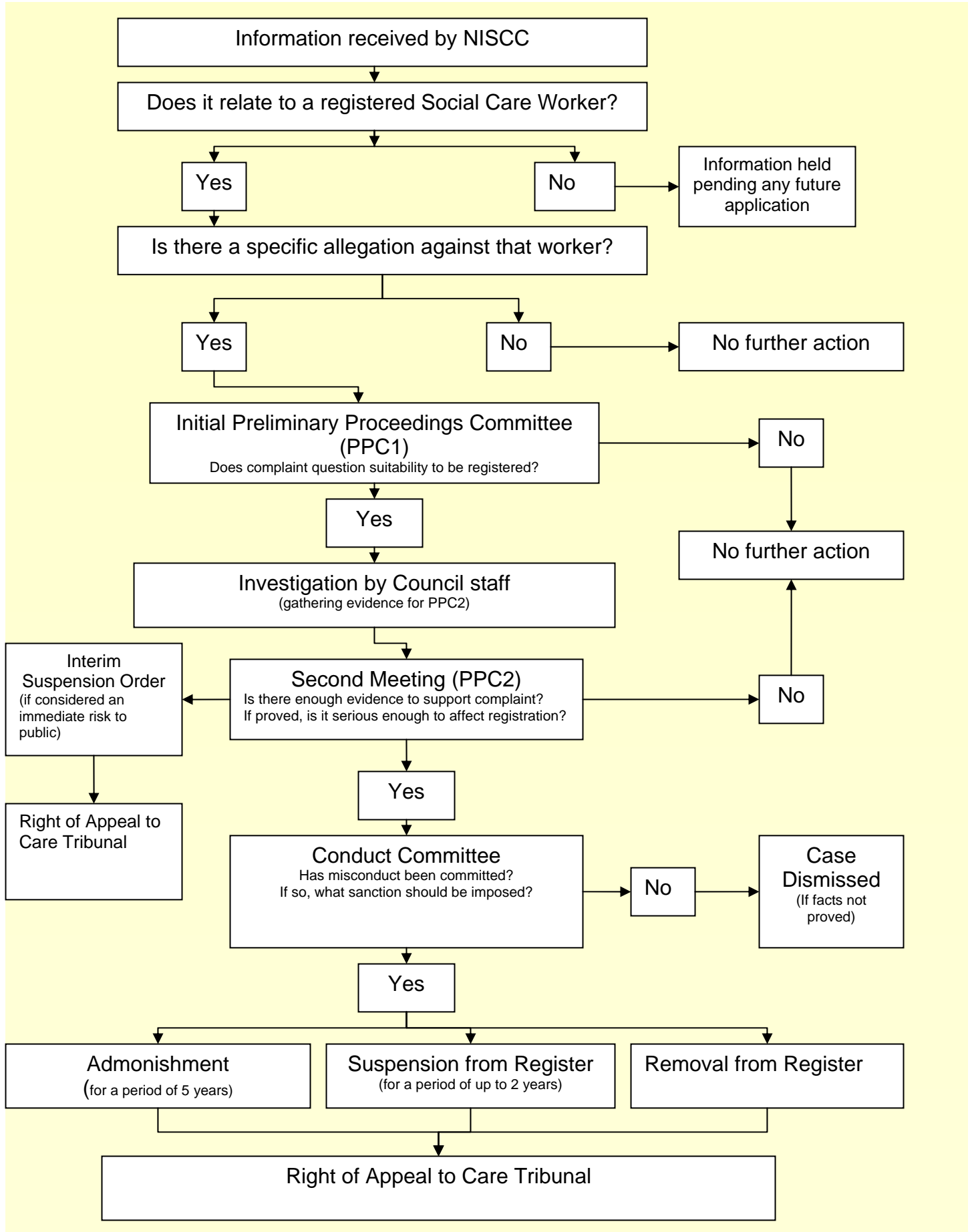
Conduct Flowchart
